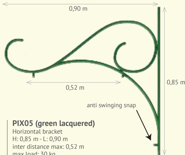
PIX05B (white lacquered) Horizontal bracket H: 0,85 m - L: 0,90 m inter distance max: 0,52 m max load: 30 kg
